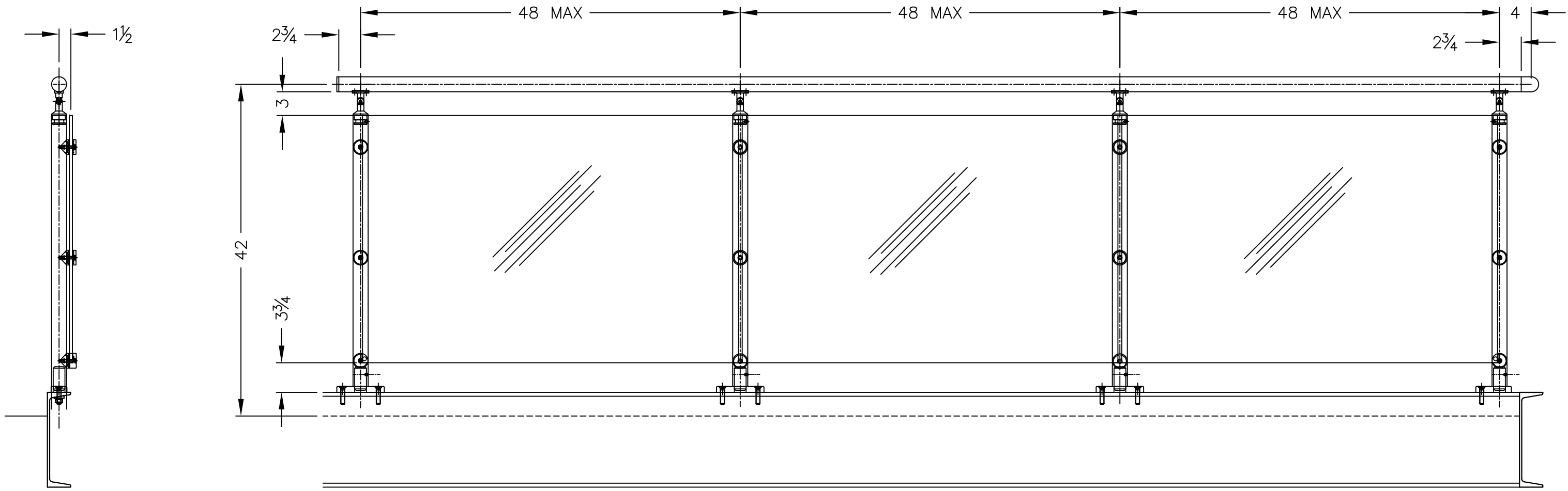
VUE RAIL - LEVEL (STRINGER MTG.) GUARD RAIL
