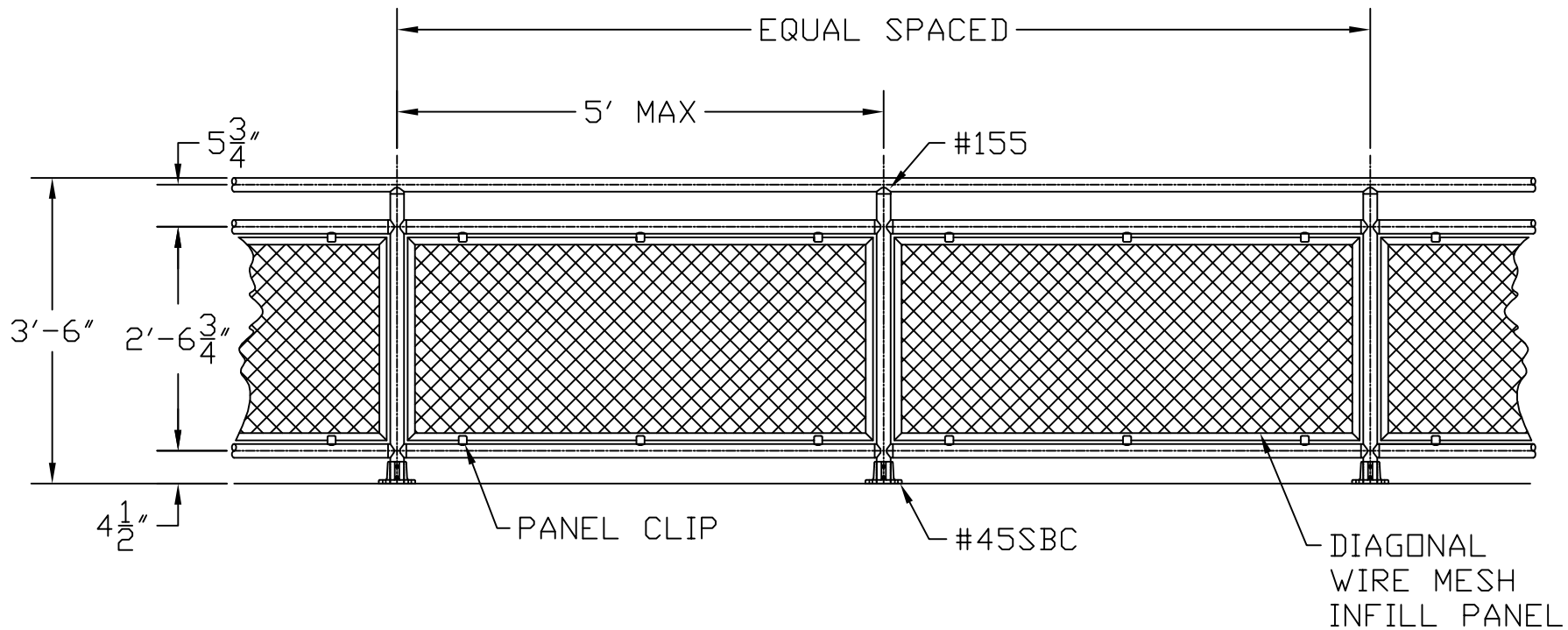
TYPICAL LEVEL HANDRAIL WITH INFILL INTERNA-RAIL DETAIL
