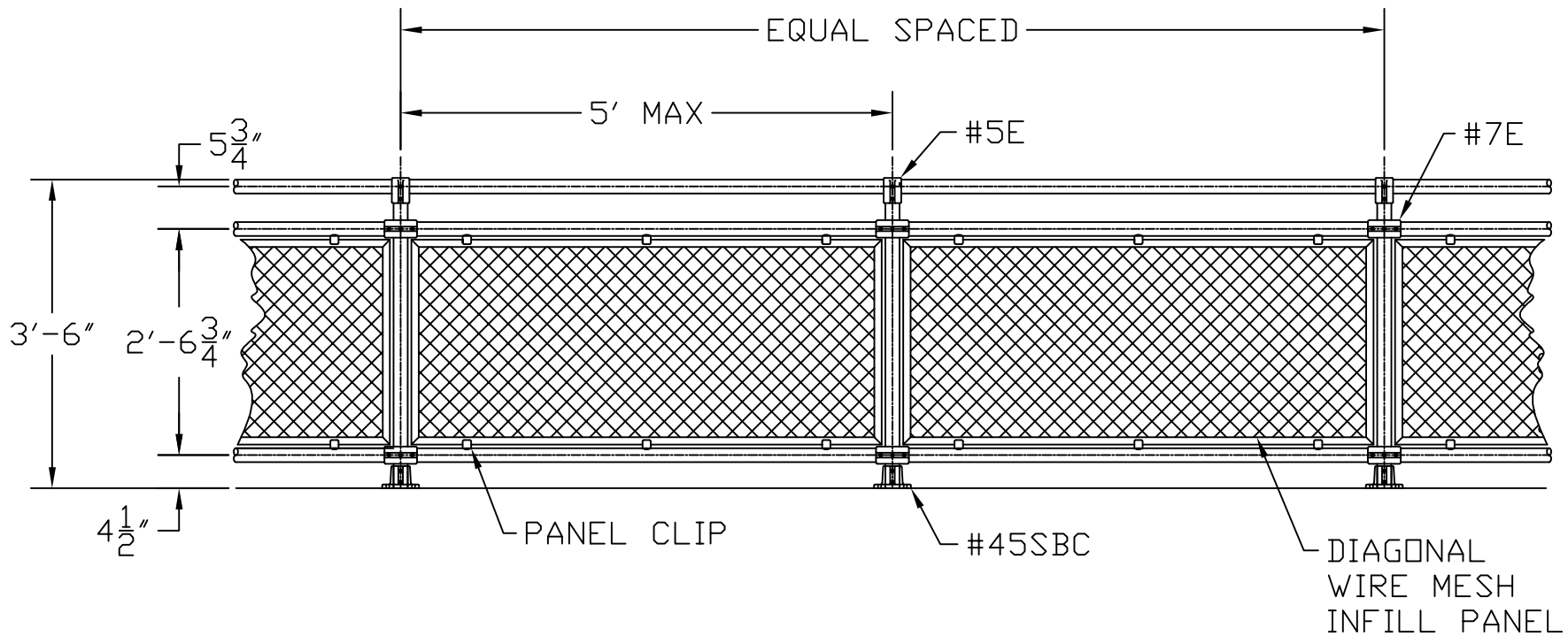
TYPICAL LEVEL HANDRAIL WITH INFILL SPEED RAIL DETAIL
